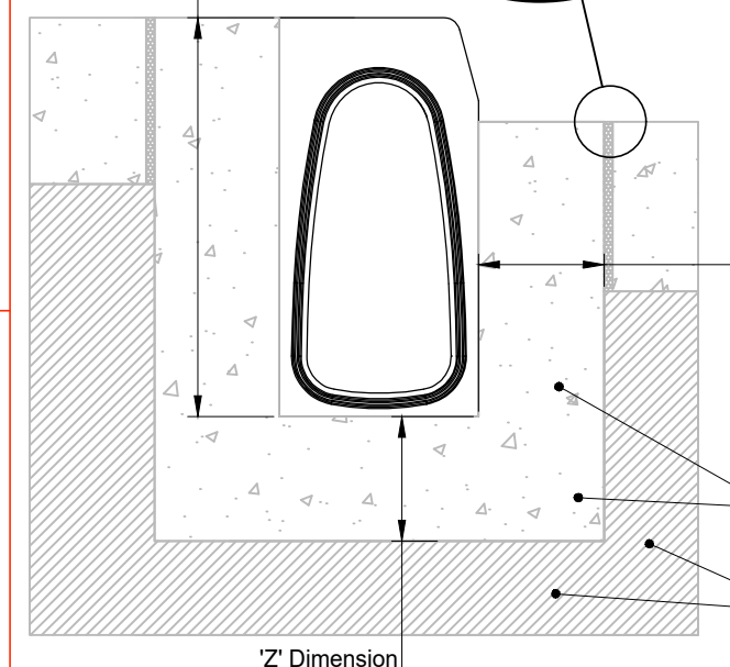
1 : 10 ACO KerbDrain KDHB Concrete Pavement
