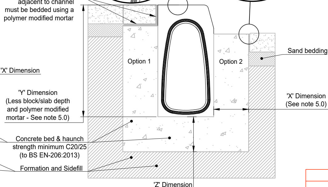
1 : 10 ACO KerbDrain KDHB Block Pavement (Option 1 and 2)
