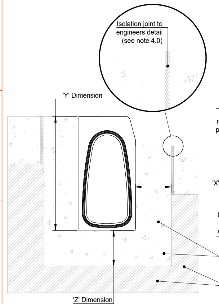
1 : 10 ACO KerbDrain KDHB Concrete Pavement
