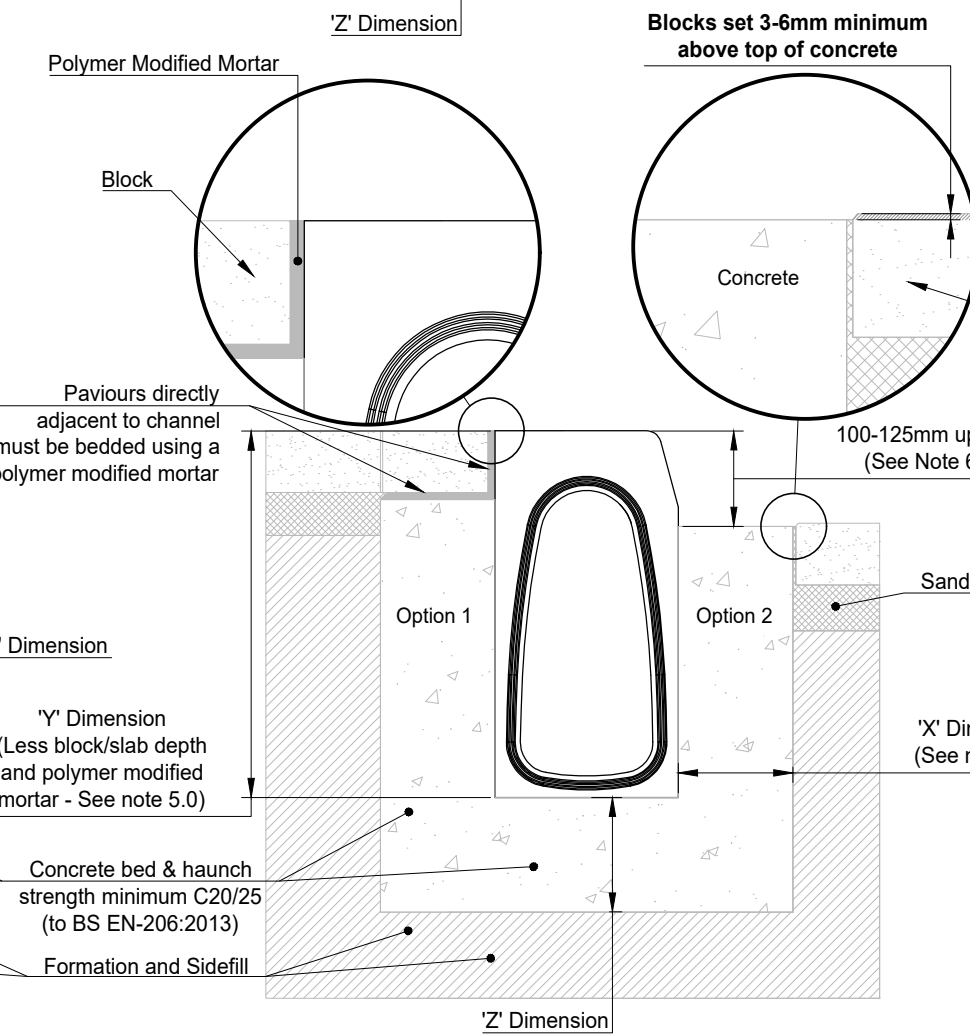
1 : 10 ACO KerbDrain KDHB Block Pavement (Option 1 and 2)
