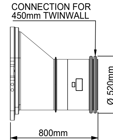
ACO Qmax 700 MALE END CHAMBER CONNECTOR
