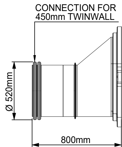
ACO Qmax 700 FEMALE END CHAMBER CONNECTOR
