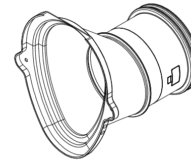
ISOMETRIC VIEW MALE END CHAMBER CONNECTOR
