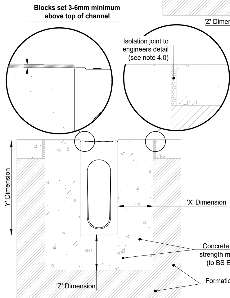
1 : 10 ACO RoadDrain Concrete Pavement
