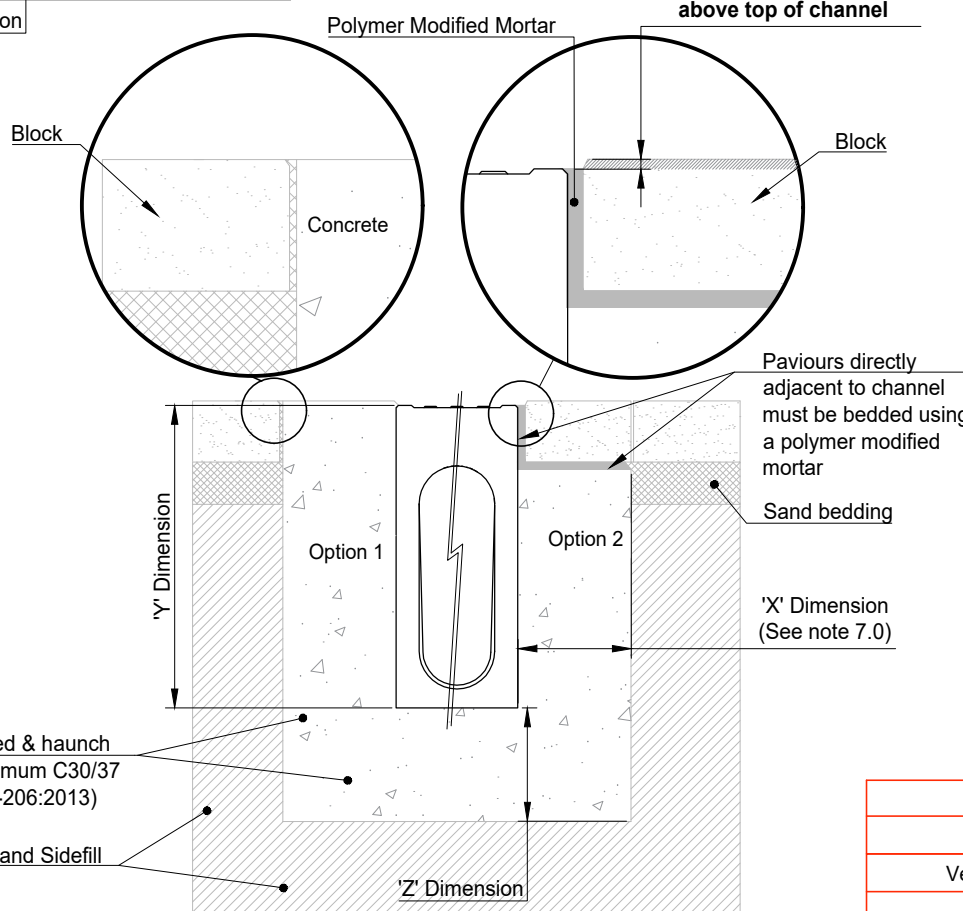
1 : 10 ACO RoadDrain Block Pavement (option 1 and 2)
