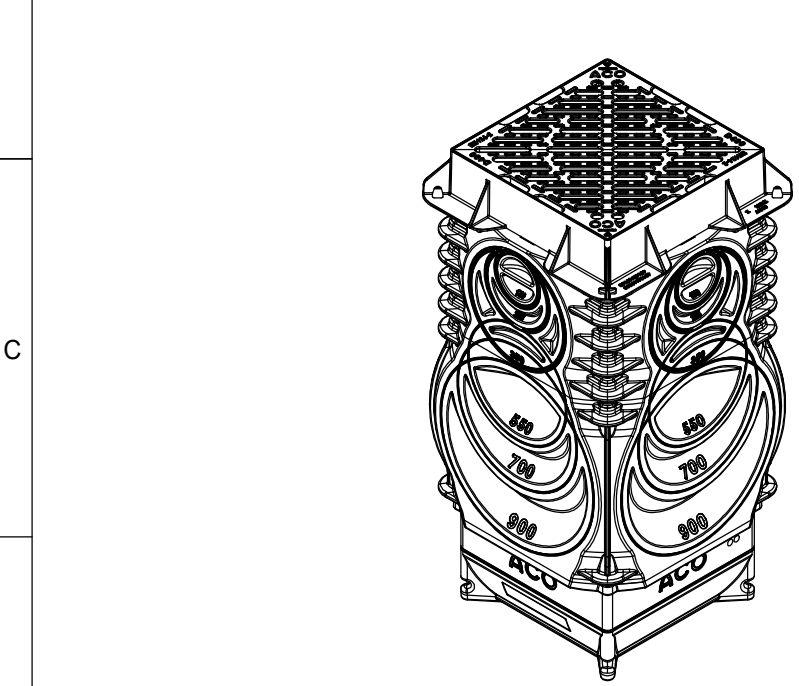
ISOMETRIC VIEW SCALE 1:20
