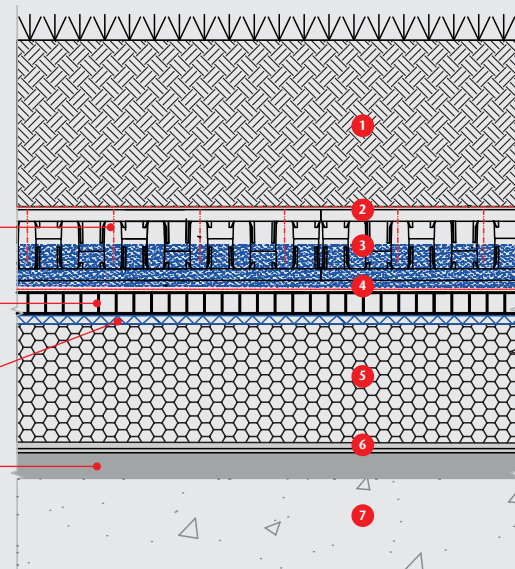
Inverted blue green roof with flow restrictor
